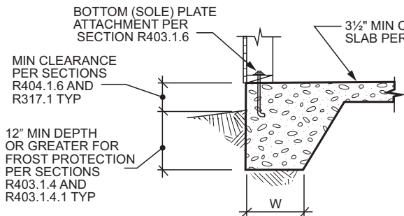
1 MONOLITHIC SLAB-ON-GROUND WITH TURNED-DOWN FOOTING SCALE: NOT TO SCALE
